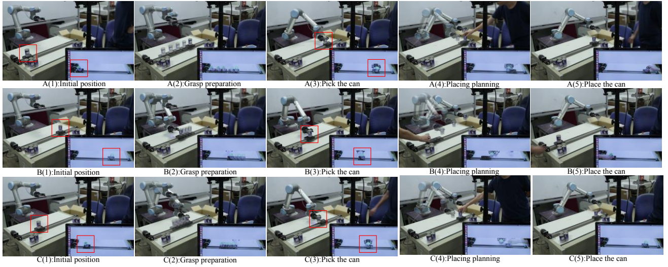
Fig. 22. The steps of robot picking and placing cans on the outward phase (A,C) and the returning phase(B). The target is enclosed by a red frame.
