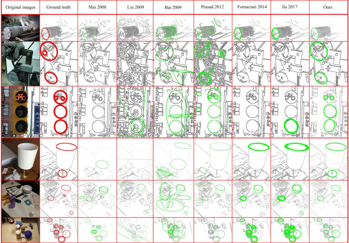
Fig. 14. The detection practical examples for Dataset HX(the first three rows) and Dataset DHX (the last three rows).
