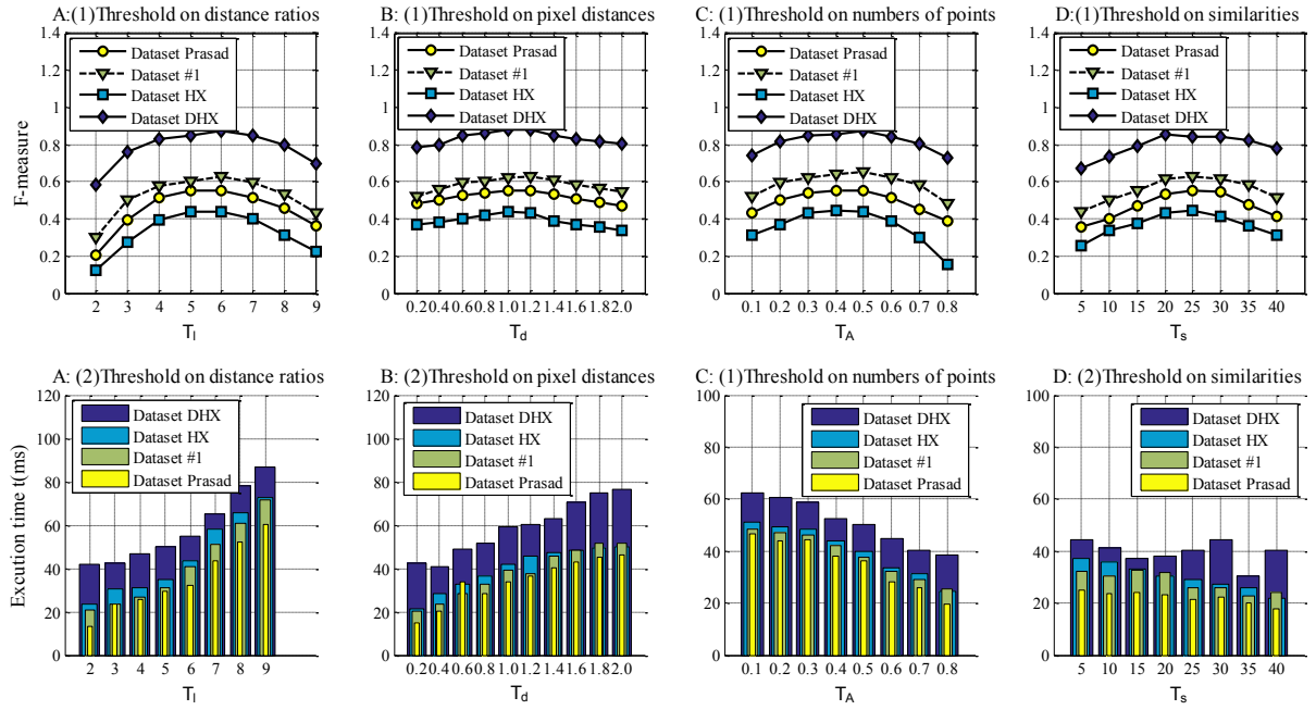
Fig. 12. The effectiveness values and execution times for four thresholds T_l, T_d, T_\psi, T_s .
