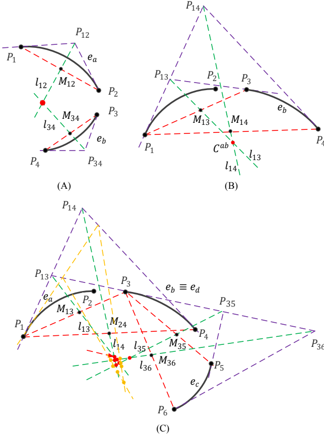
Fig. 6. Illustration of the calculation method of the elliptic center. The methods of estimating the elliptic center proposed by others (A) and us (B, C). The red line segments are the two longest ones in all line segments (B). P_i denotes endpoints of arcs e_a, e_b, e_c ; P_{ij} represents the intersection of the tangent lines through P_i and P_j . M_{ij} is the midpoint of the line segment P_iP_j . l_{ij} indicates the line formed by P_{ij} and M_{ij} . The shifted intersection points (yellow dots) are formed by the shifted lines (yellow lines) joining the midpoints of the chords and the intersections of the tangent lines when the slope of the line through the midpoint P_{34} of the arc e_b is not correct due to image noise. i, j = 1, 2, 3, 4, 5, 6 .
