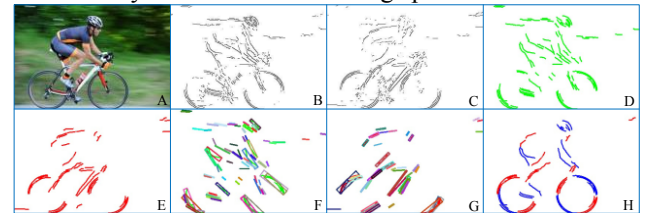
Fig. 2. An example of pre-processing. The initial image(A); the edge images along two edge directions by gradient signs (B, C); the edge images after the process of 8-connectivity(D,E); the arcs enclosed by oriented bounding boxes(F,G); the image after pre-processing(H).
