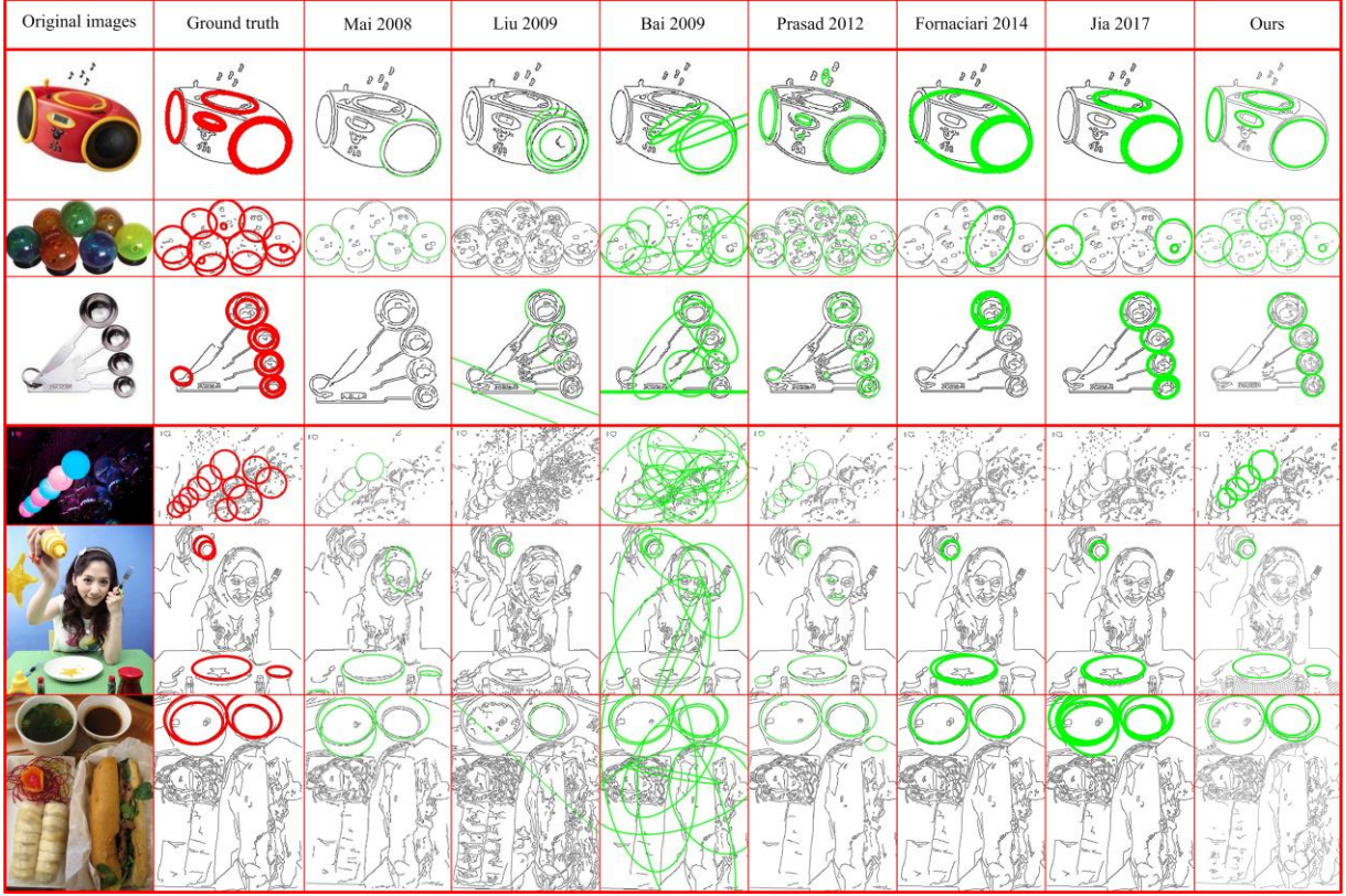
Fig. 13. The detection practical examples for Dataset Prasad (the first throw rows) Dataset #1(the last three rows).
