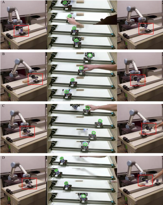
Fig. 21. The robot grasping cans on the conveyor with 4 speeds in a dynamic scenario. The target is enclosed by a red frame. The speeds of A,B,C,D are 2.5cm/s, 5.0cm/s, 7.5cm/s, 10.0cm/s, respectively. Several detection examples for each speed are shown in the middle column.
