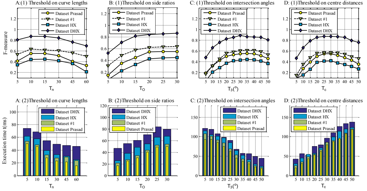
Fig. 11. The effectiveness values and execution times for four thresholds T_n, T_O, T_\theta, T_c .
