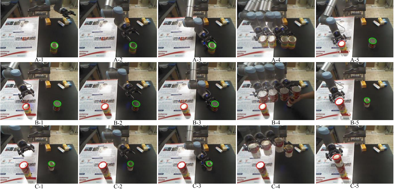
Fig. 20. Stacking food cans. Place the first can (A-1,2,3), stack the second can on the first can (B-1,2,3) and stack the third can on the second can (C-1,2,3).
