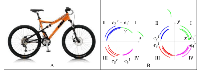
Fig. 5. Arc classification. e_i^l and e_i^r denote the left and right endpoints of an arc.
