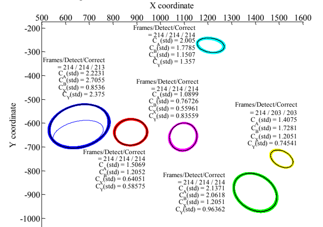
Fig. 16. Statistic results of detecting six ellipses in a video stream.
