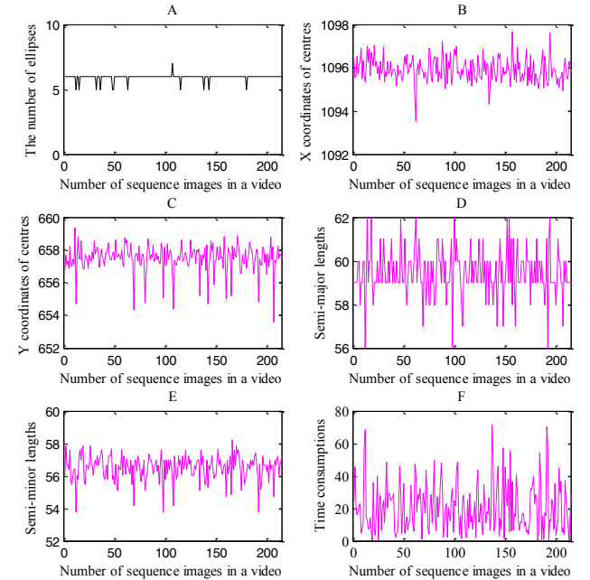
Fig. 17. Detailed detection performance in all image frames for one of the objects. (F) shows the execution time for each image.
