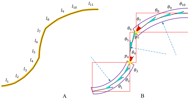
Fig. 3. A curve fitted by a series of line segments (A); an arc extraction by splitting an arc at a change of direction of curvature p_4 and a large change of curvature p_7 . Line segments with arrows represents the directions of curvatures of arcs and the red rectangle frames denote bounding boxes enclosing arcs extracted.
